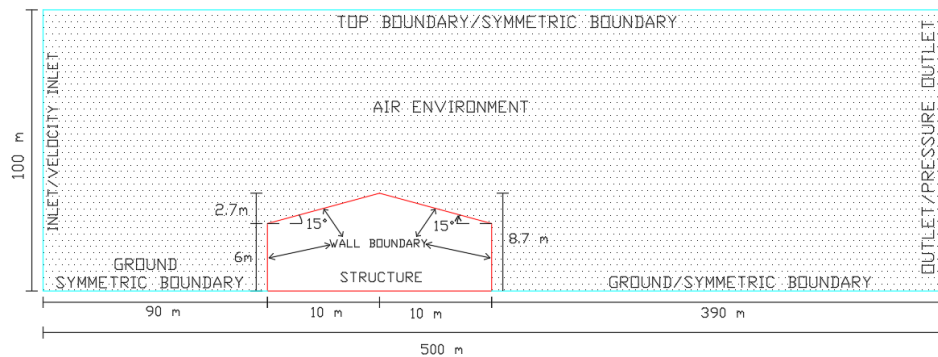
Figure 7. Dimensions and boundary conditions of building flow field
