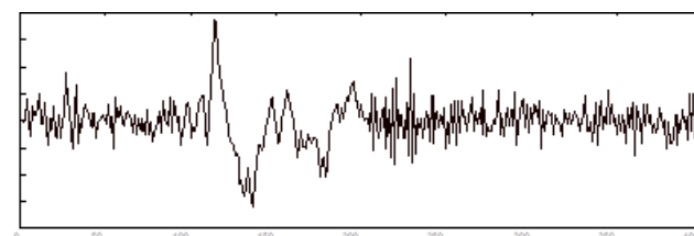
Figure 6. Residues for case \lambda = .99 in RWLS method.
