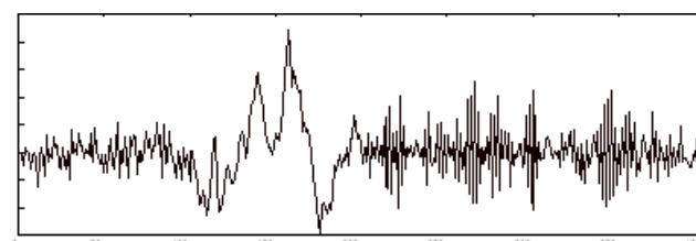
Figure 3. Residues for case \lambda = 1 in RWLS method.
