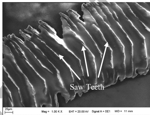
Figure 8. Saw tooth formation at 0.3 mm/rev.
