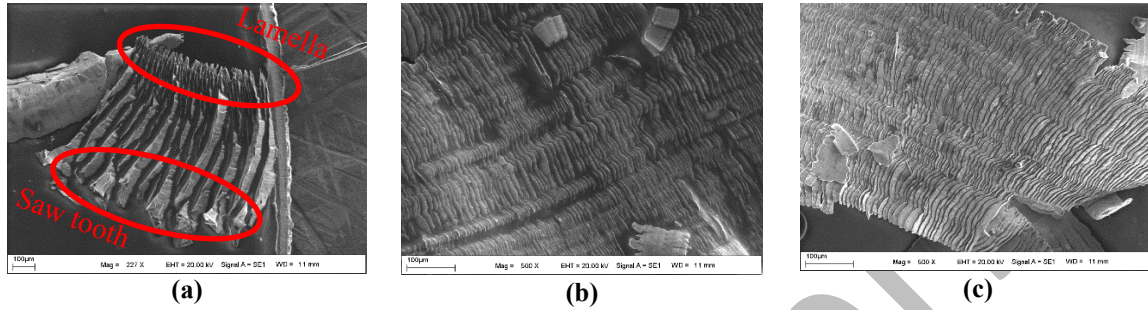
Figure 10. Lamella structure formation at; a) transition of saw teeth and lamella structure, b) 0.3 mm/rev, c) 0.2 mm/rev.
