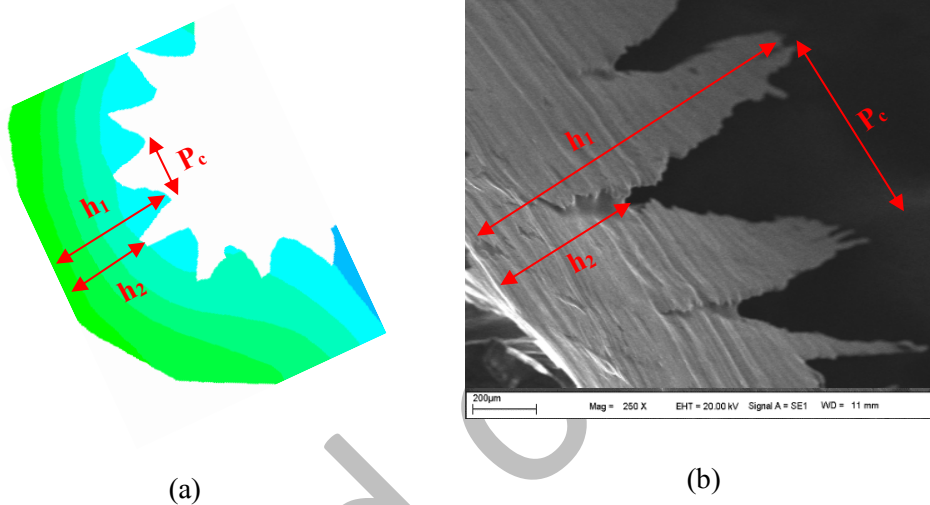
Figure 12. Comparison of modeled and experimental chip; a) modelled chip, b) experimental chip.
