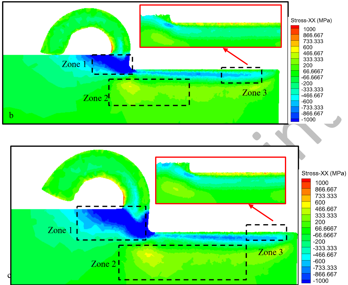
Figure 14. Formation mechanism of residual stress; a) f=0.1 mm/rev, b) f=0.2 mm/rev, c) f=0.3 mm/rev
