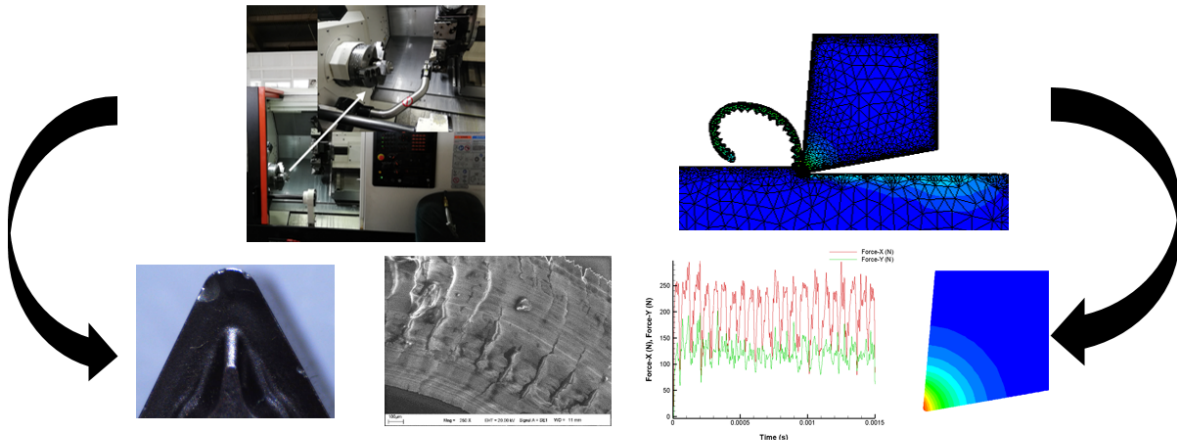
Figure 1. Machining procedure.
