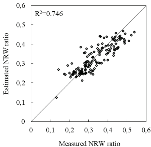
Figure 7. Scatter graph for WSQ/NJ-NL-WM model.
