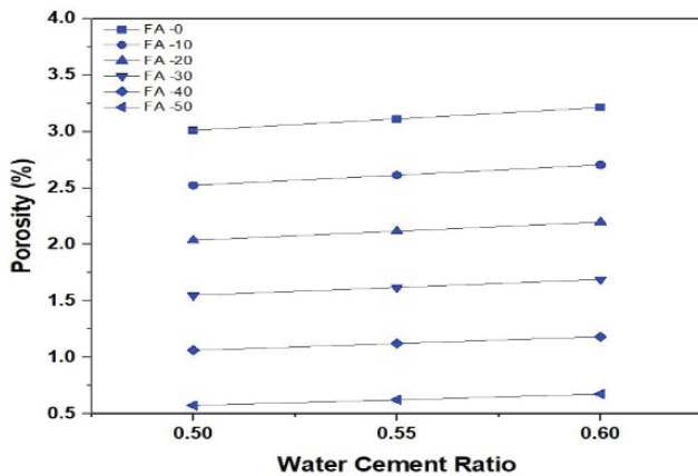
Figure 8. Binder content 300kg/m 3 , w/c vs Porosity.
