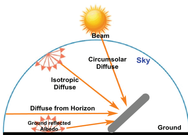
Figure 1. Diffuse component of the global solar radiation.
