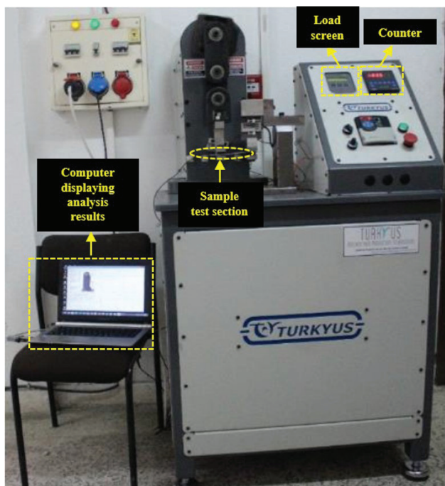
Figure 4. Schematic view of the flexural fatigue test system specially designed for this study and test machine image.
