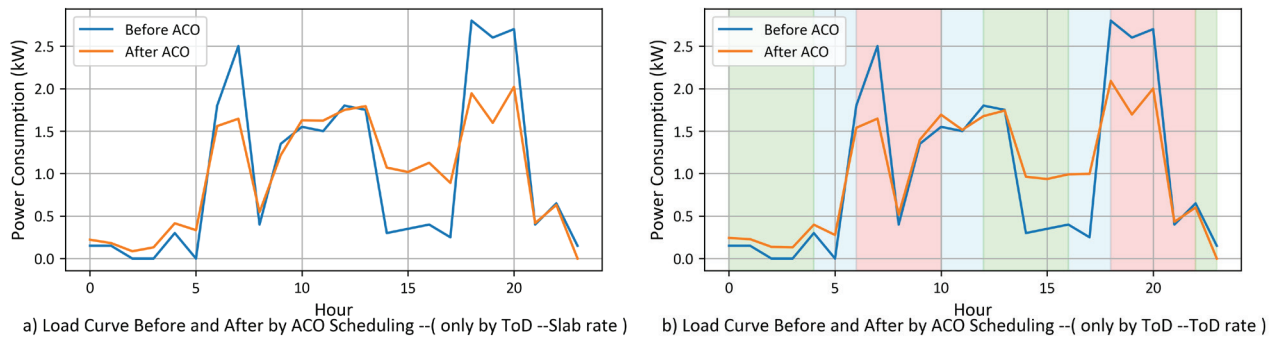
Figure 5. Load curve Before and After Scheduling load by ACO a) Slab rate b) ToD rate.
