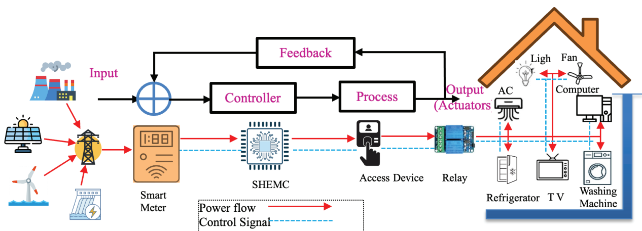
Figure 1. Workflow of Smart home energy management system.
