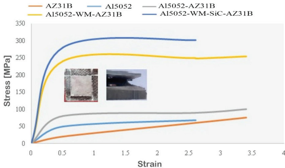
Figure 10. Stress-strain curve.
