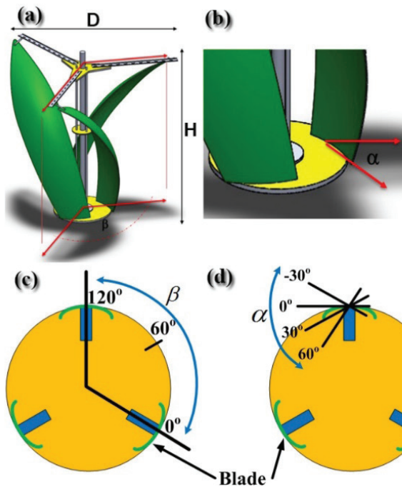
Figure 8. Variation of aspect ratio (AR), \beta angle, \alpha angle; (a) shows the ratio of AR can be varied by D and H length, representing the \beta angle between blades; (b) shows the \alpha angle of each blade.
