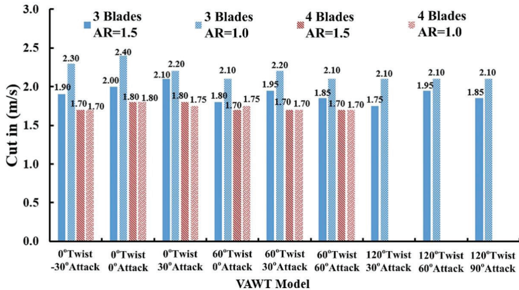
Figure. 11 VAWT model and cut-in wind speed of 3 Blades with AR=1.5, 3 Blades with AR=1.0, 4 Blades with AR=1.5 and 4 Blades with AR=1.0 that were varied the Twist and Attack angle of VAWT Model.
